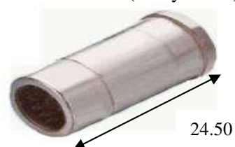
00.4 252.000 Accelerator Shaft Bush 00.4252 BR (Bronze) 00.4252 AS (Alloy Steel)
